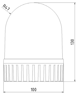
LED universal rotating- and flashing light orange/anthracite 24V AC/DC and/or 230V AC Ref.: 905.RLSL.20
