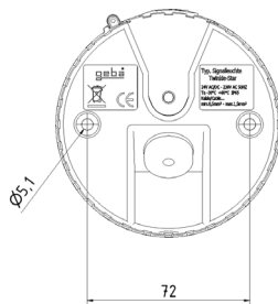
LED universal rotating- and flashing light orange/anthracite 24V AC/DC and/or 230V AC Ref.: 905.RLSL.20
