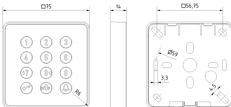
Cody Touch-Silver-black LED-Blue Ref.: 507.BT21.03
